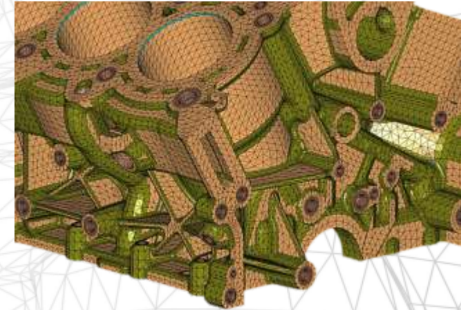
Tetra Mesh
